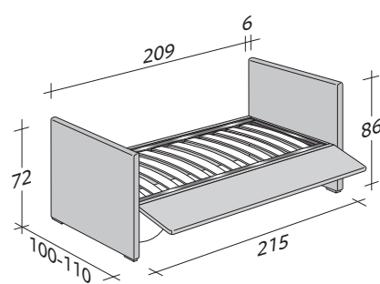
BISS 1ST BED ADJUSTABLE SLATTED BASE VERSION C : HIGH HEADBOARD - LOW FOOTBOARD
