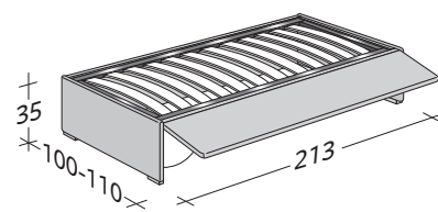
BISS 1ST BED ADJUSTABLE SLATTED BASE VERSION F : NO HEADBOARD - NO FOOTBOARD
