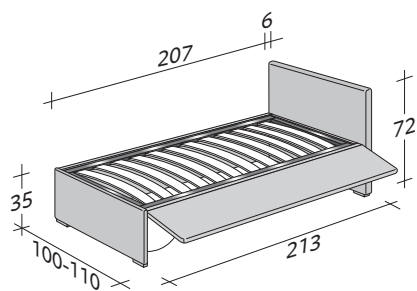
BISS 1ST BED ADJUSTABLE SLATTED BASE VERSION D : LOW HEADBOARD
