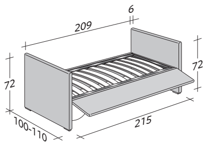
BISS 1ST BED ADJUSTABLE SLATTED BASE VERSION E : LOW HEADBOARD - LOW FOOTBOARD
