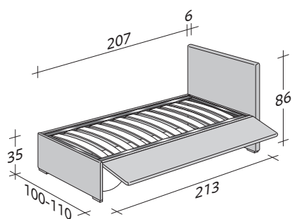
BISS 1ST BED ADJUSTABLE SLATTED BASE VERSION A : HIGH HEADBOARD
