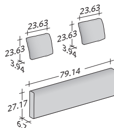
BACKRESTS WITH CUSHIONS WITH BAND FOR BACKREST
