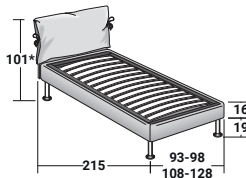
BASE H16 ADJUSTABLE SLATTED BASE ELECTRICALLY POWERED ADJUSTABLE SLATS
