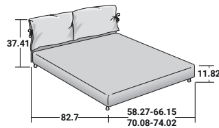
RIGID BASE
