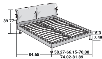
BASE H16 ADJUSTABLE SLATTED BASE ELECTRICALLY POWERED ADJUSTABLE SLATS
