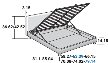
STORAGE BASE ADJUSTABLE SLATTED BASE
