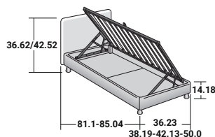
STORAGE BASE SIDE OPENING ADJUSTABLE SLATTED BASE
