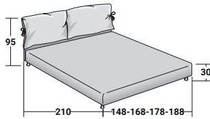
RIGID BASE
