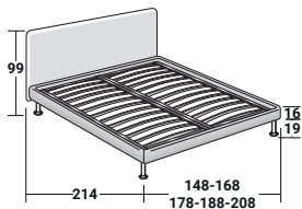
BASE H16 ADJUSTABLE SLATTED BASE ELECTRICALLY POWERED ADJUSTABLE SLATS
